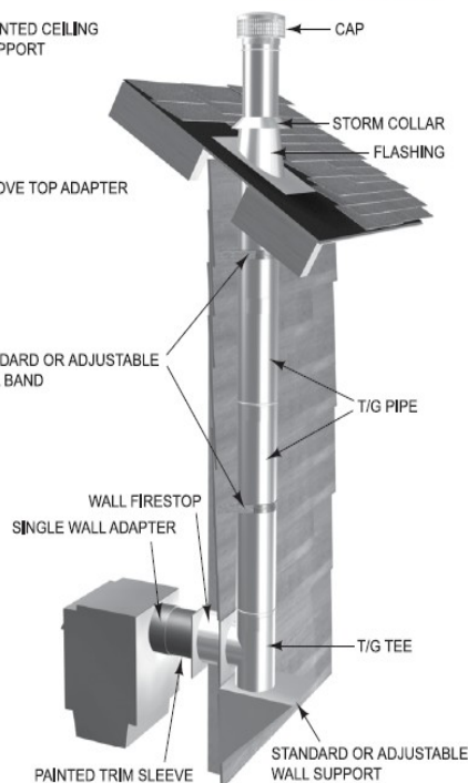
Typical Installation Drawings
