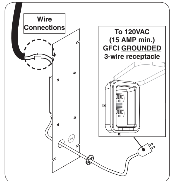
Fig. 20-2 Connect: Wires, Plate, Power
