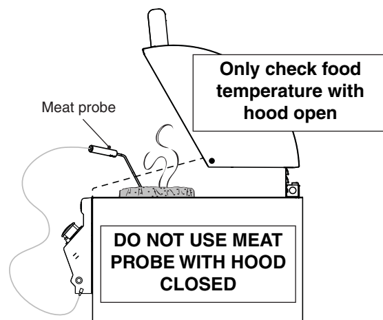
Fig. 27-3 Meat probe
