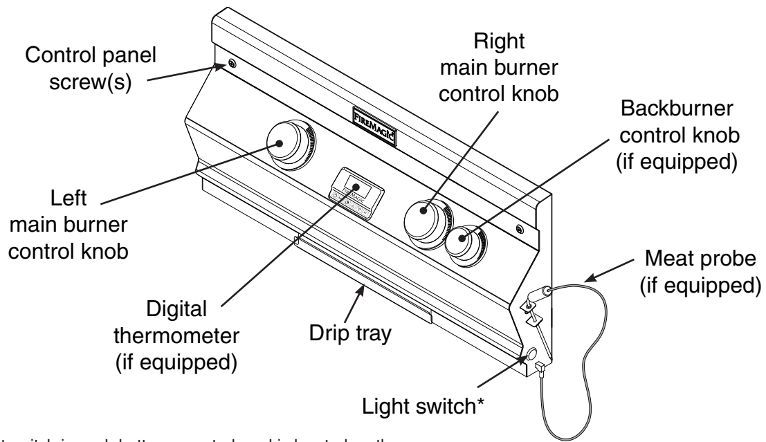
Fig. 23-1 A430s controls
