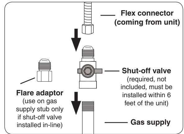
Fig. 20-1 Connecting to a gas line
