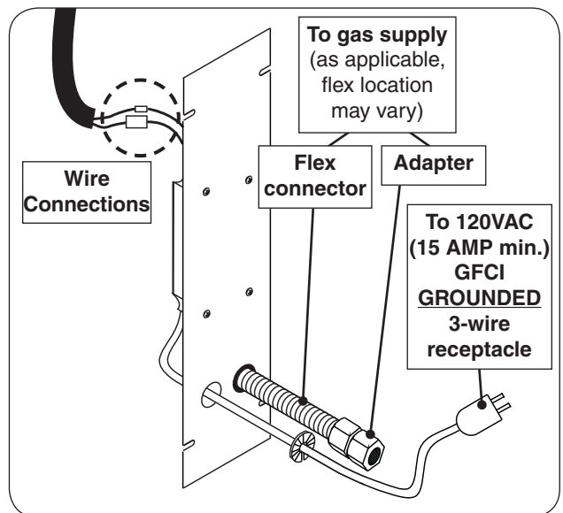
Fig. 17-1 Connect: Gas, Wires, Plate, Power
