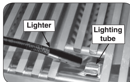
Fig. 25-2 - Manual lighting
