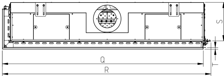
Plan View
