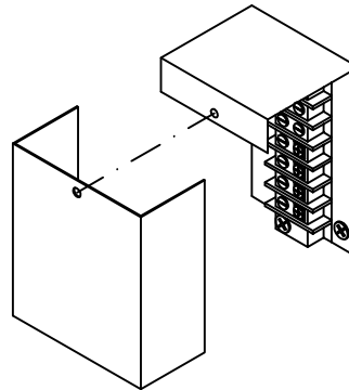
99.12.01.N TERMINAL BLOCK ASSEMBLY
