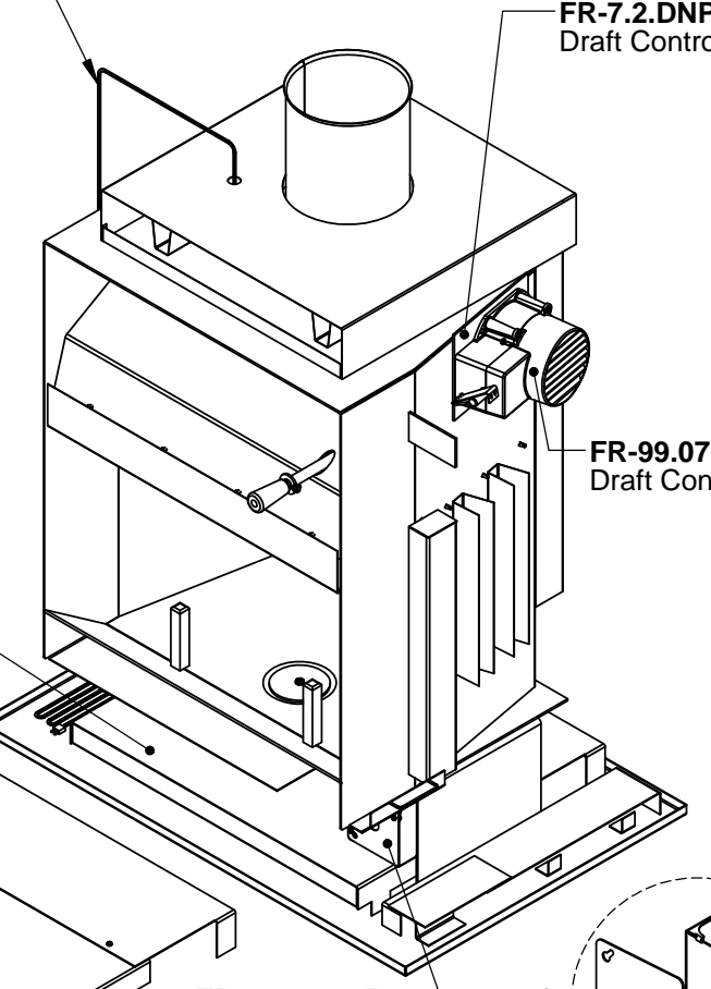
FR-99.12.01.P Terminal Block
