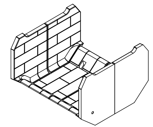
99.11.01.R COMPLETE REFRACTORY BRICKS SET
