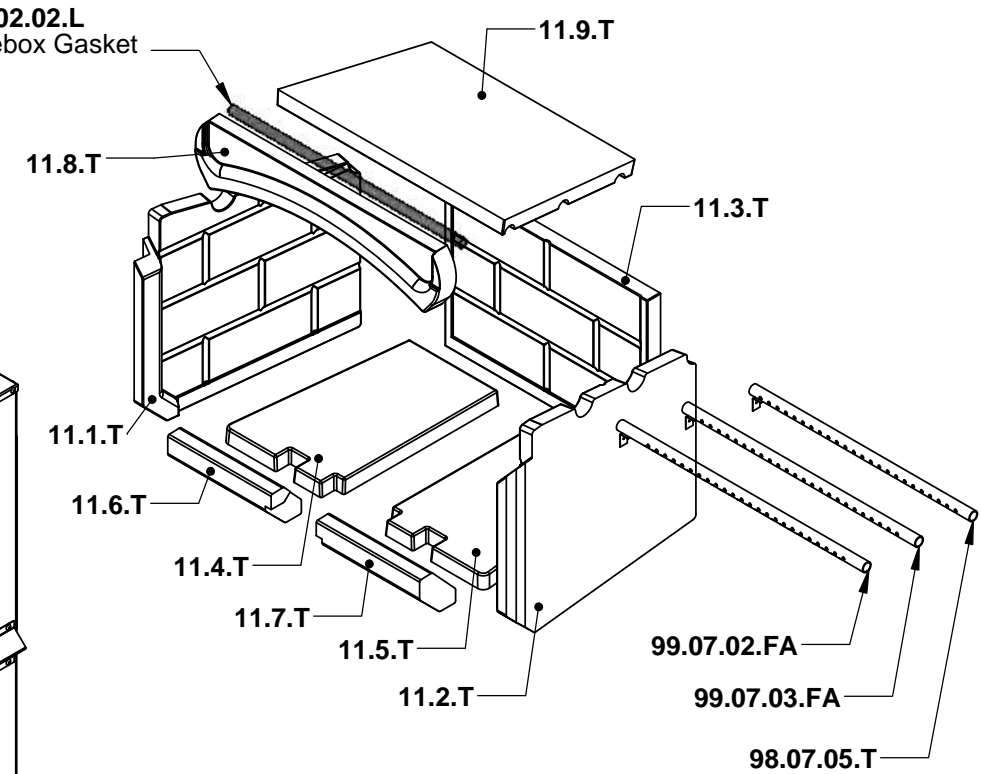
99.11.01.T Complete Refractory Brick Set
